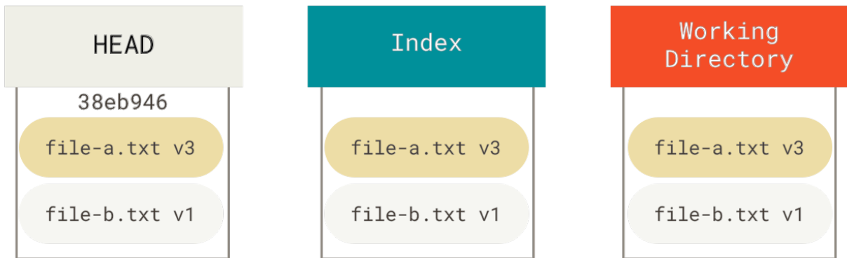
Figure 151. Git repository
